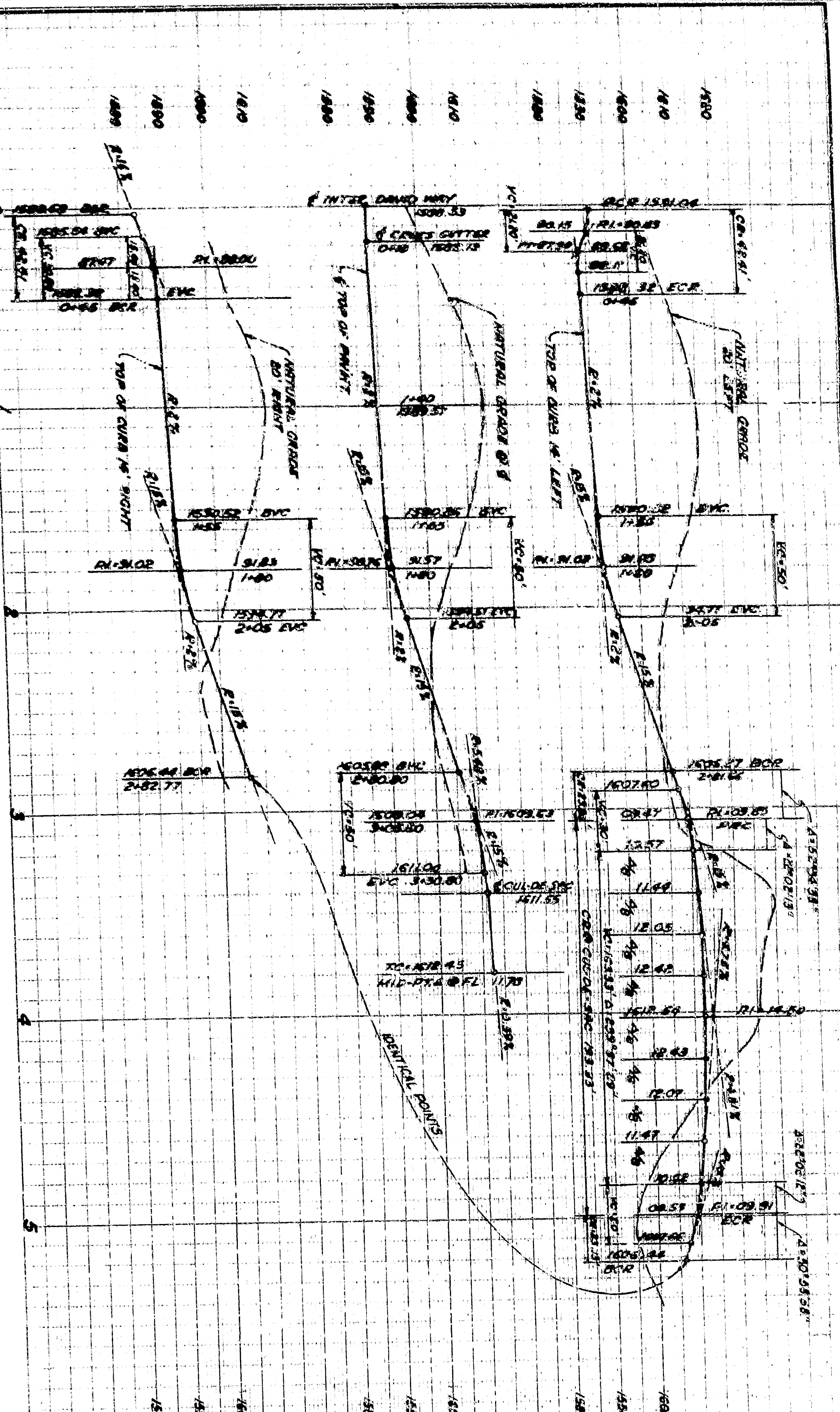
PROFILE - PONDEROSA DRIVE SCALE: HORIZONTAL 1" = 40' VERTICAL 1" = 20'
