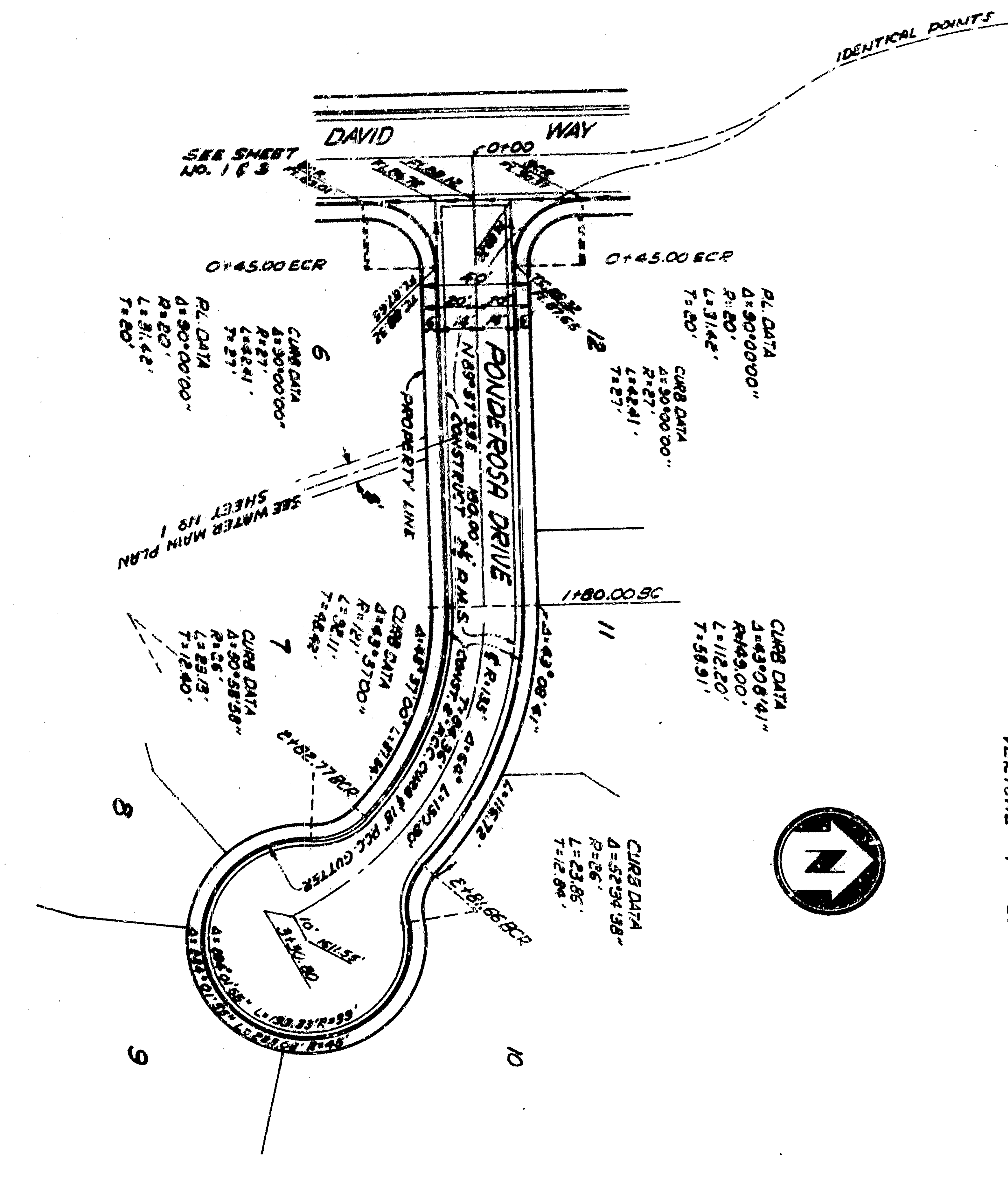
PLAN - PONDEROSA DRIVE SCALE: 1" = 40'
